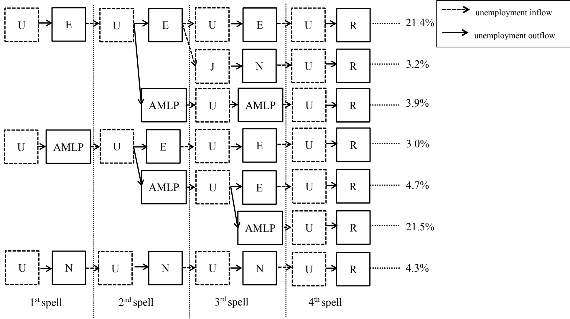
Figure 4. The 4-spell transitions pathways of at least 3% of observations
