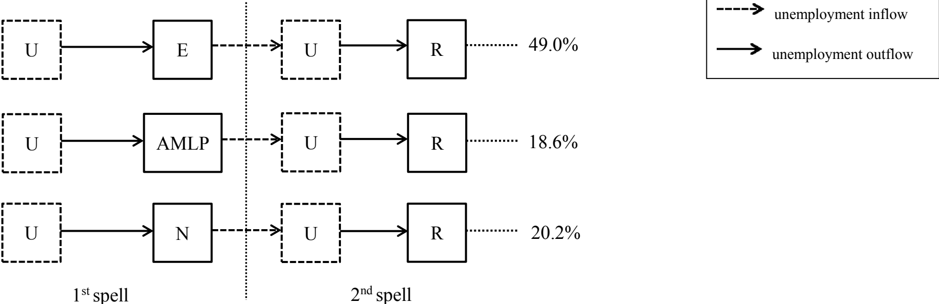
Figure 2. The 2-spell transitions pathways of at least 10% of observations
