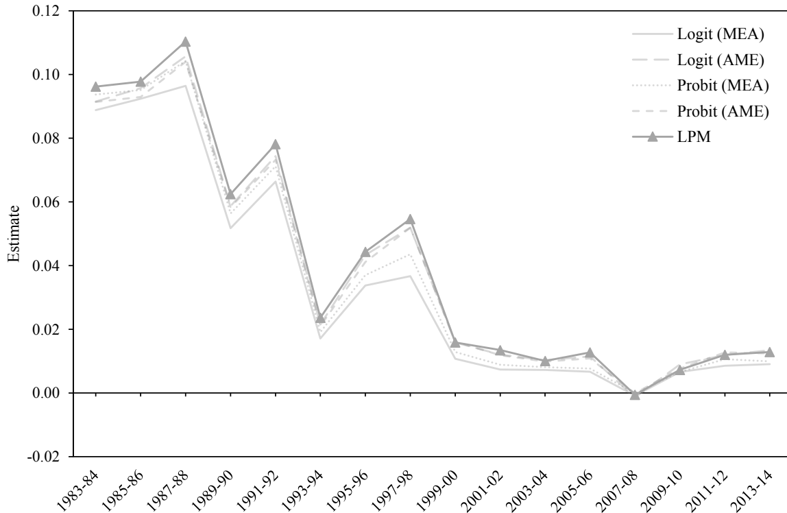
FIGURE E.1: CONDITIONAL UNEMPLOYMENT DIFFERENTIALS, BY ESTIMATION METHOD: CHS
