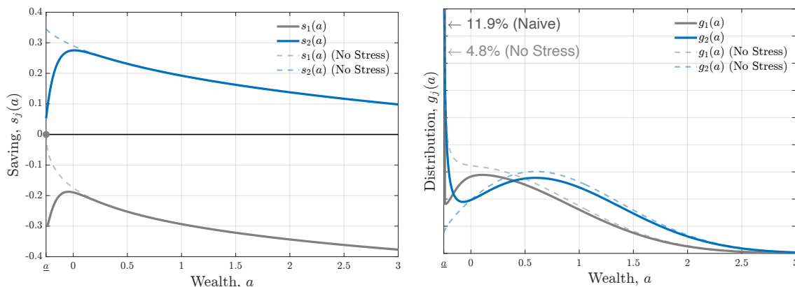
Figure E.15: Stressed Spending (Naivete).
