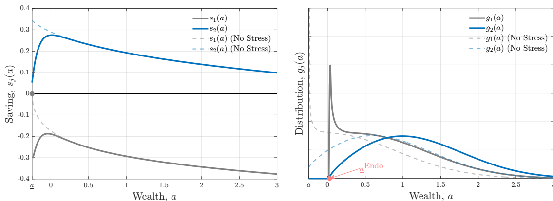
Figure E.14: Stressed Spending (Sophistication).
