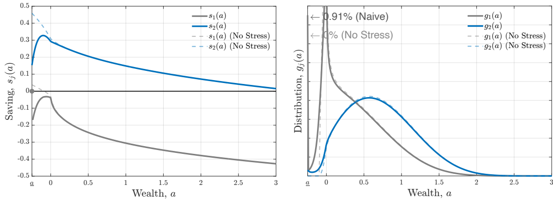
Figure E.13: Different Saving and Borrowing Rates (Naivete, \kappa = 6\% ).
