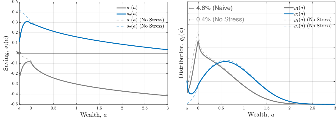
Figure E.12: Different Saving and Borrowing Rates (Naivete, \kappa = 4\% ).
