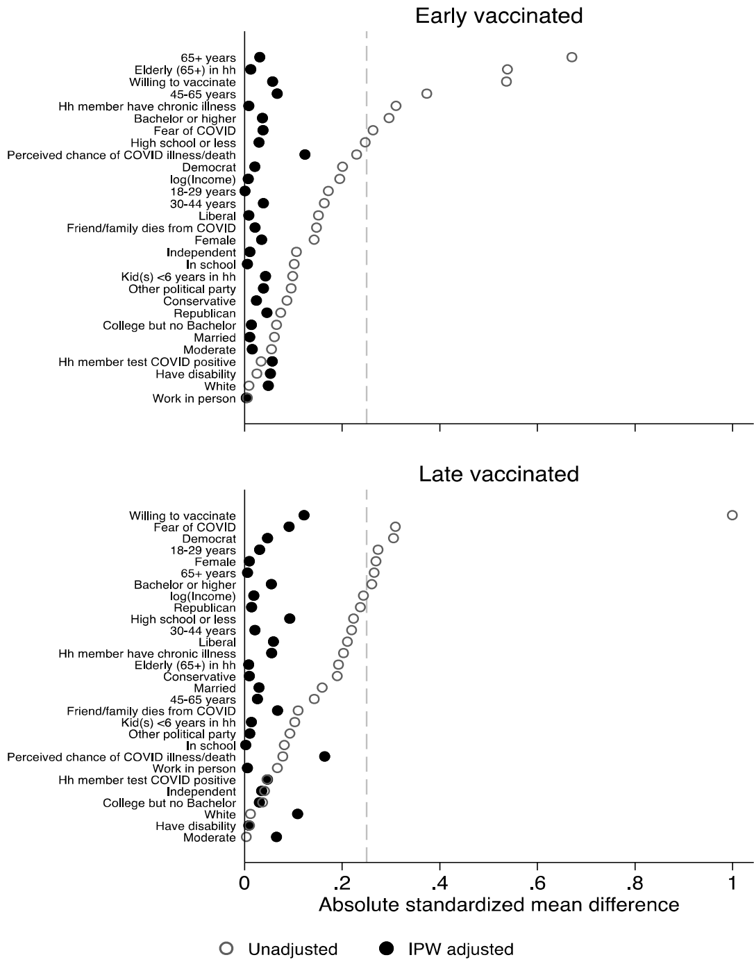
Figure 3 A check for balance in covariates between vaccinated and unvaccinated individuals using the absolute standardized mean difference with and without IPW adjustment for early and late vaccinated.
