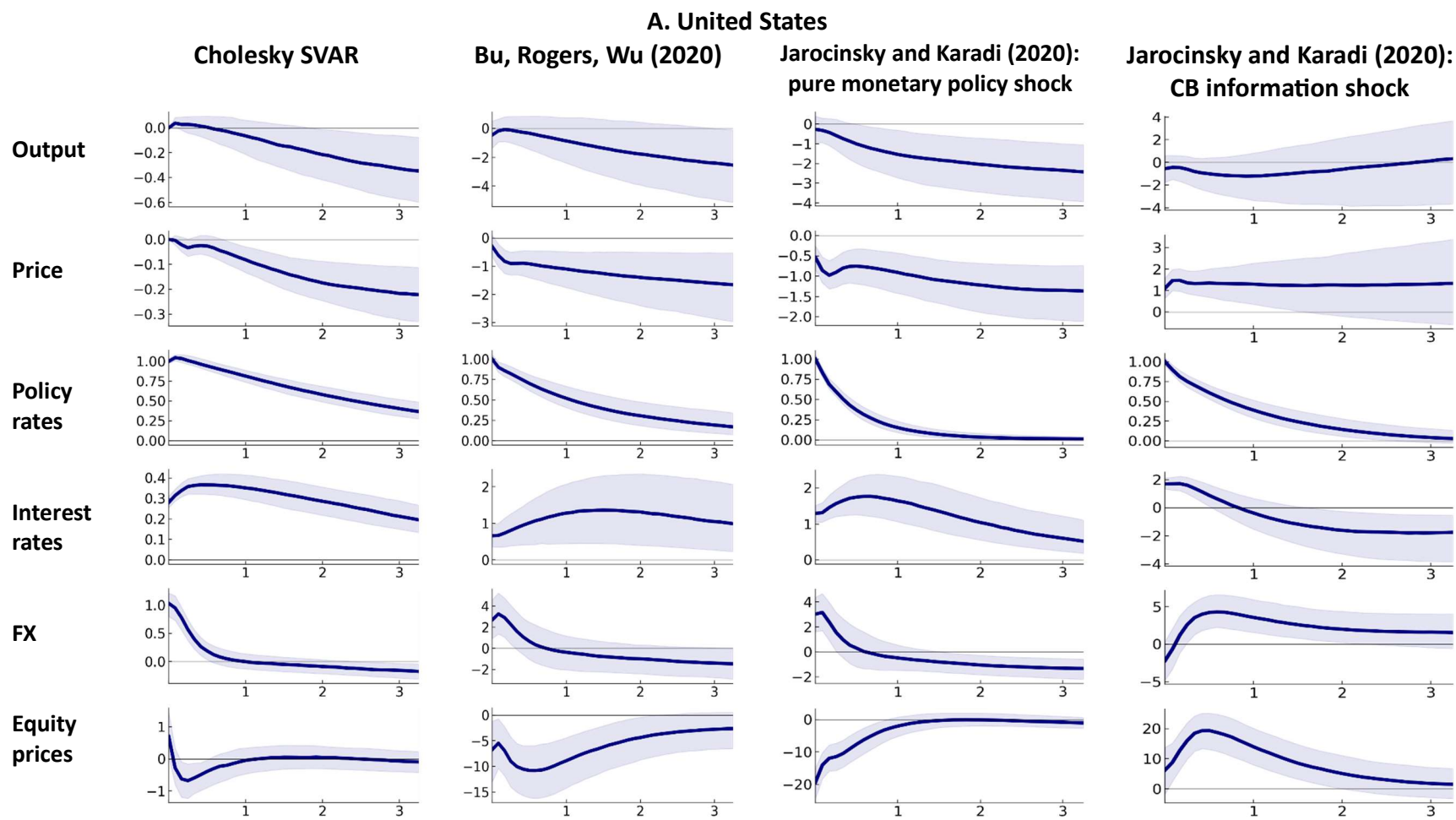
Figure A5. Impulse responses to a monetary policy tightening: Cholesky VAR with expectations
